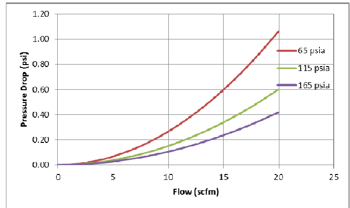
Figure 1 – Pressure Drop versus Flow
