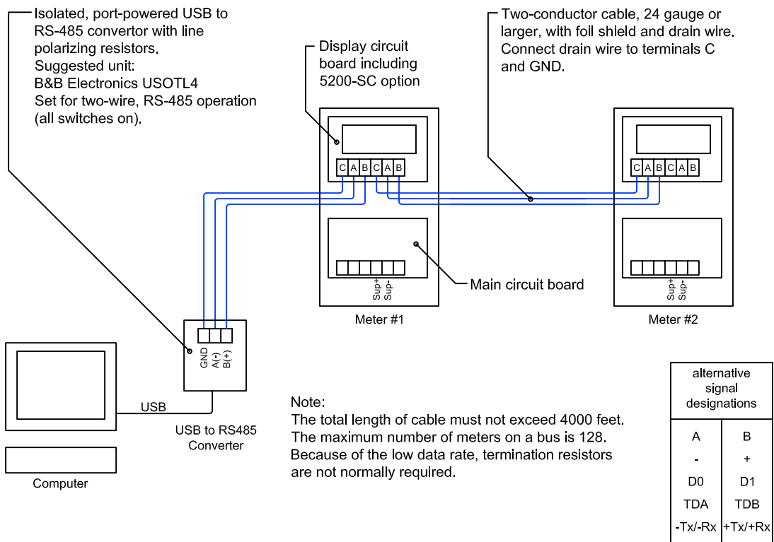
Figure 1 Basic RS-485 Signal Wiring
